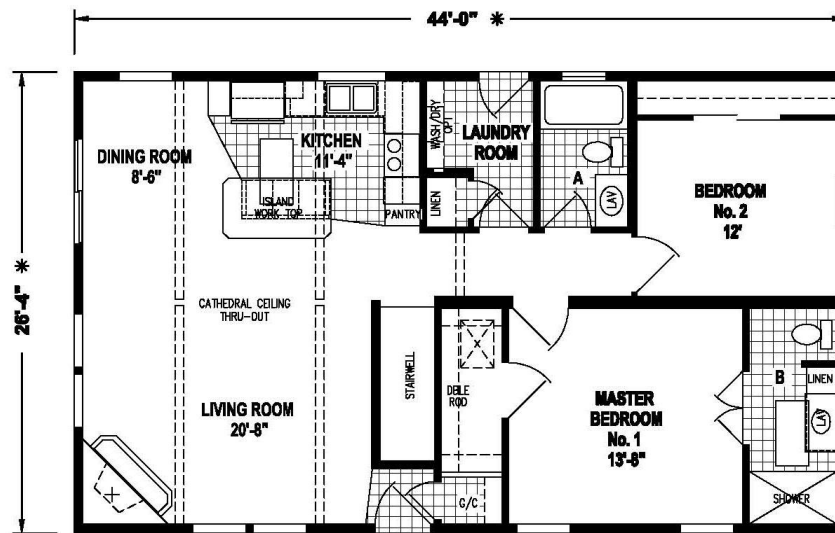
A236MT/4428 (1,158 SQ.FT.) 2BEDROOM - 2BATHS - CATHEDRAL THRU-OUT
